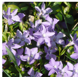
Vinca minor
